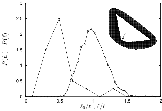
FIG. 3: Histograms of the distributions of normalized distances of dynamically generated (full circles) and randomly sampled (open circles) points in the sets \mathcal{S} for \mu = 0.01 . The inset shows a two dimensional cross section of a high dimensional solution set. The dynamically constructed force state is marked by the arrow. The white area belongs to \mathcal{S} , while outside \mathcal{S} the gray scale indicates the violation of the Coulomb condition (darker means smaller violation).
